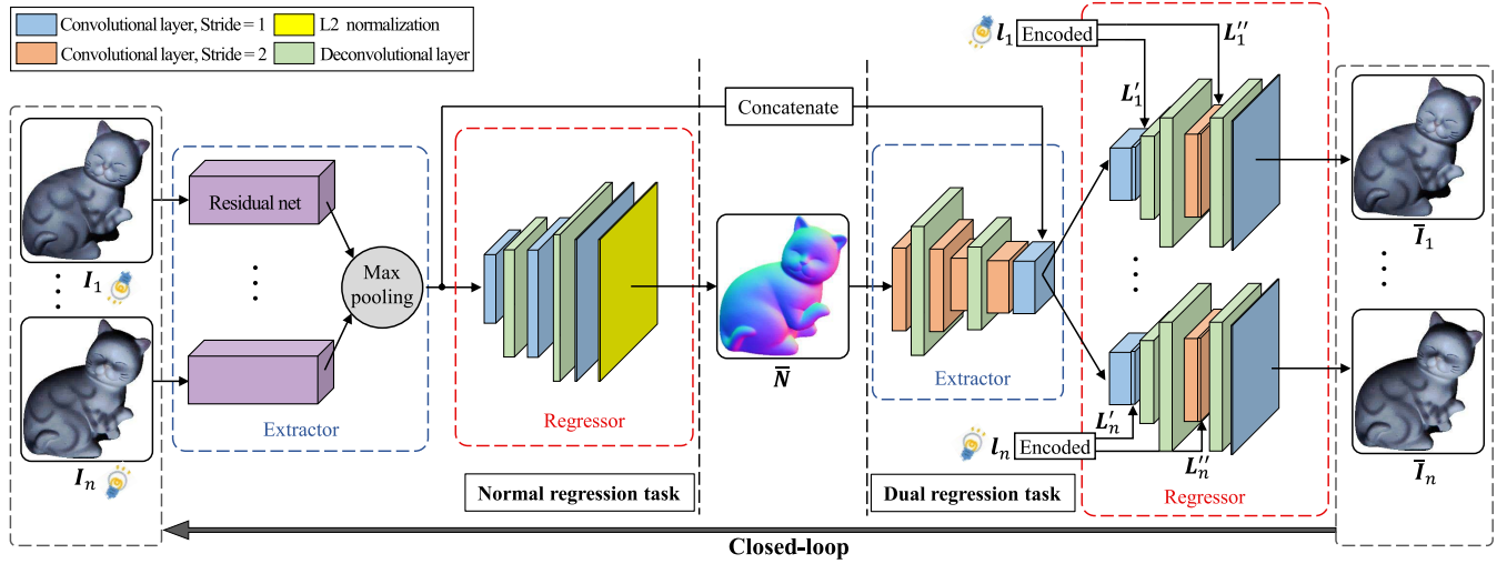
Fig. 3. The details of DR-PSN. The normal regression task estimates the surface normal, while the dual regression task synthesizes each of the reconstructed images \{\tilde{I}_1, \tilde{I}_2, \dots, \tilde{I}_n\} from the estimated surface normal \tilde{N} of the normal regression network. We concatenate the high-dimensional feature from the normal regression task to the dual regression task with a shortcut. To better regress images under specified illumination directions, we also fuse the encoded illumination directions L'_i, L''_i with the regressor twice for a corresponding reconstructed image.
